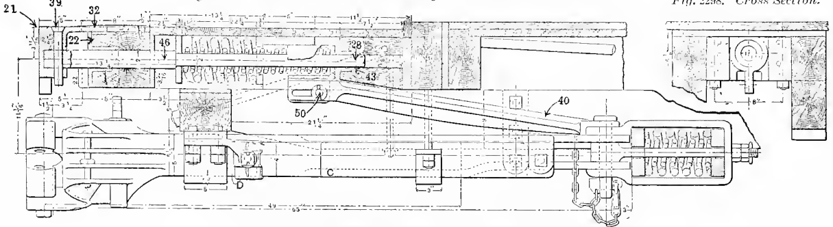
Fig. 2297. Longitudinal Section through Side Buffer-stem.
